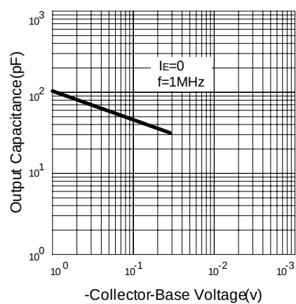
Fig.4 Collector Output capacitance
