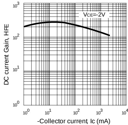
Fig.7 DC current gain
