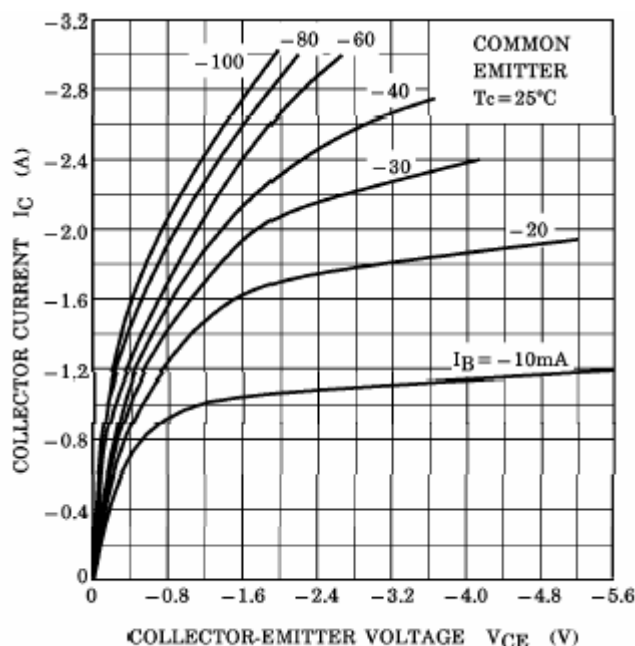
Fig.3 Static Characteristic
