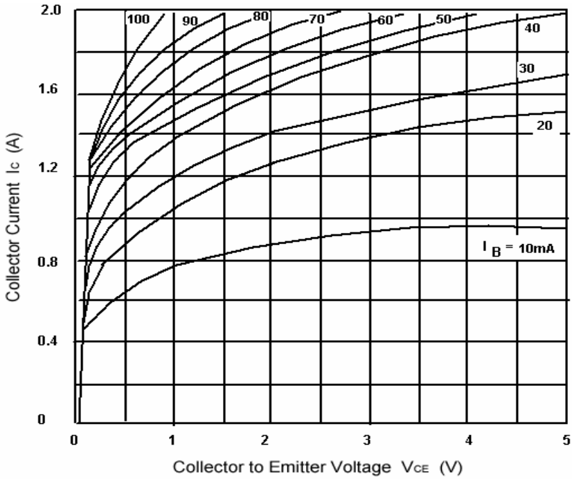
Fig.4 Static Characteristic
