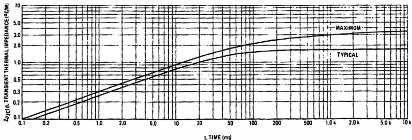
FIGURE 10 THERMAL RESPONSE
