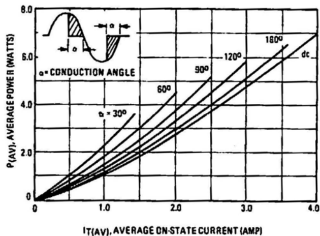
FIGURE 3 - POWER DISSIPATION
