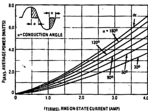
FIGURE 4 - POWER DISSIPATION
