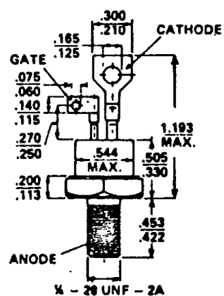
TO-48D
