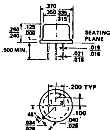
TO-39
