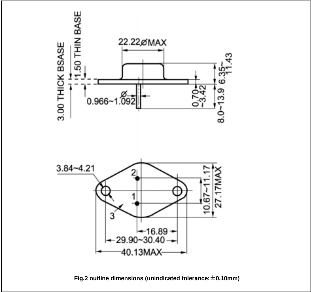
PACKAGE OUTLINE
