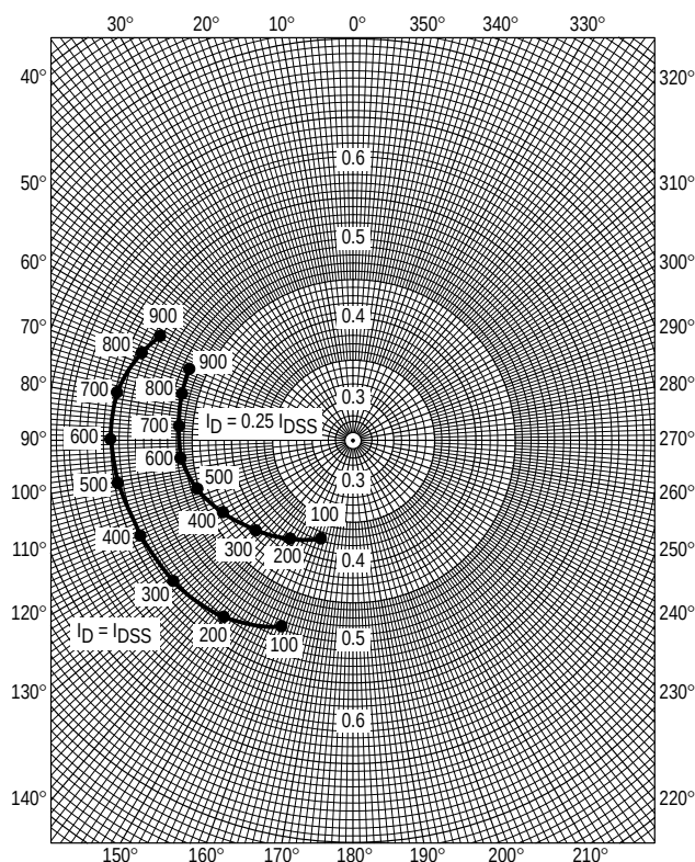
Figure 12. S_{21s}
