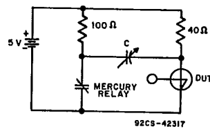
Fig. 12—Turn-off time test circuit.
