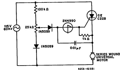
Fig. 16—Motor speed control circuit.
