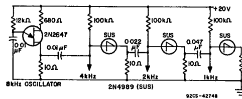
Fig. 22—Frequency divider chain circuit.
