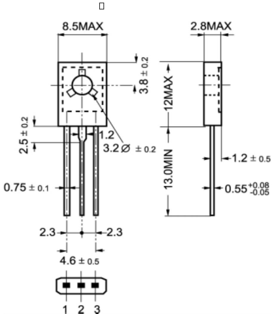
Fig.2 Outline dimensions
