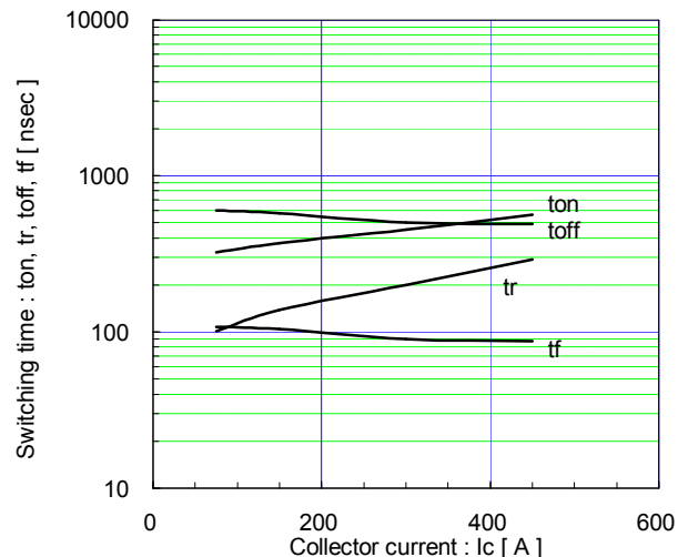
Switching time vs. Collector current (typ.) Vcc=600V, VGE=±15V, RG=2.0Ω, Tj=125°C
