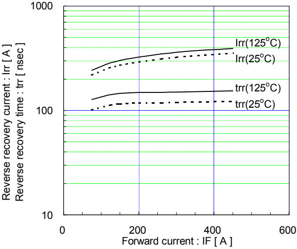
Reverse recovery characteristics (typ.) Vcc=600V, VGE=±15V, RG=2.0Ω
