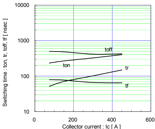
Switching time vs. Collector current (typ.) Vcc=600V, VGE=±15V, RG=2.0Ω, Tj=25°C
