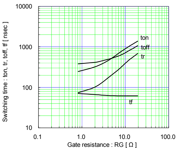
Switching time vs. Gate resistance (typ.) Vcc=600V, Ic=300A, VGE=±15V, Tj=25°C
