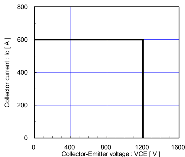
Reverse bias safe operating area (max.) +VGE=15V, -VGE ≤ 15V, RG ≥ 2.0Ω, Tj ≤ 125°C Stray inductance ≤ 100nH
