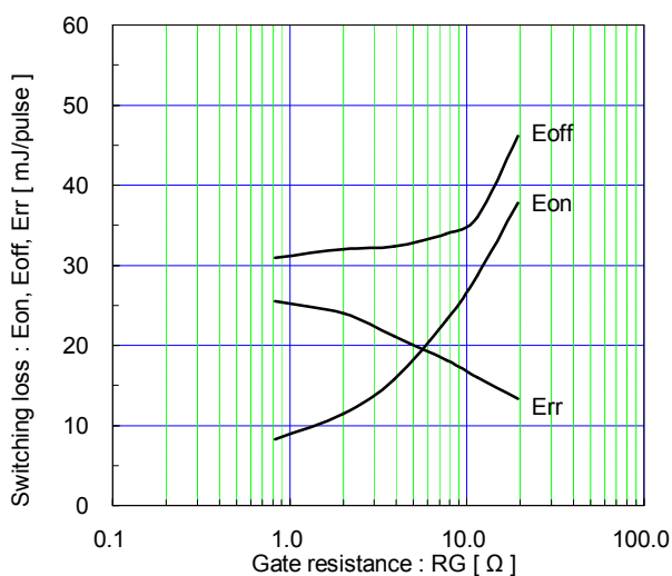
Switching loss vs. Gate resistance (typ.) Vcc=600V, Ic=300A, VGE=±15V, Tj=125°C
