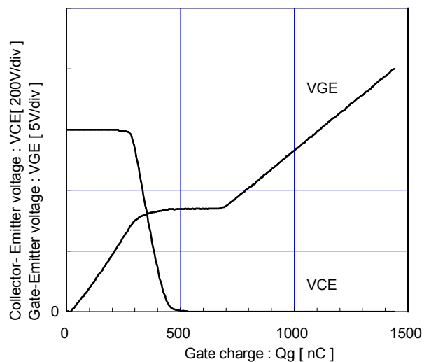
Dynamic Gate charge (typ.) Vcc=600V, Ic=300A, Tj=25°C
