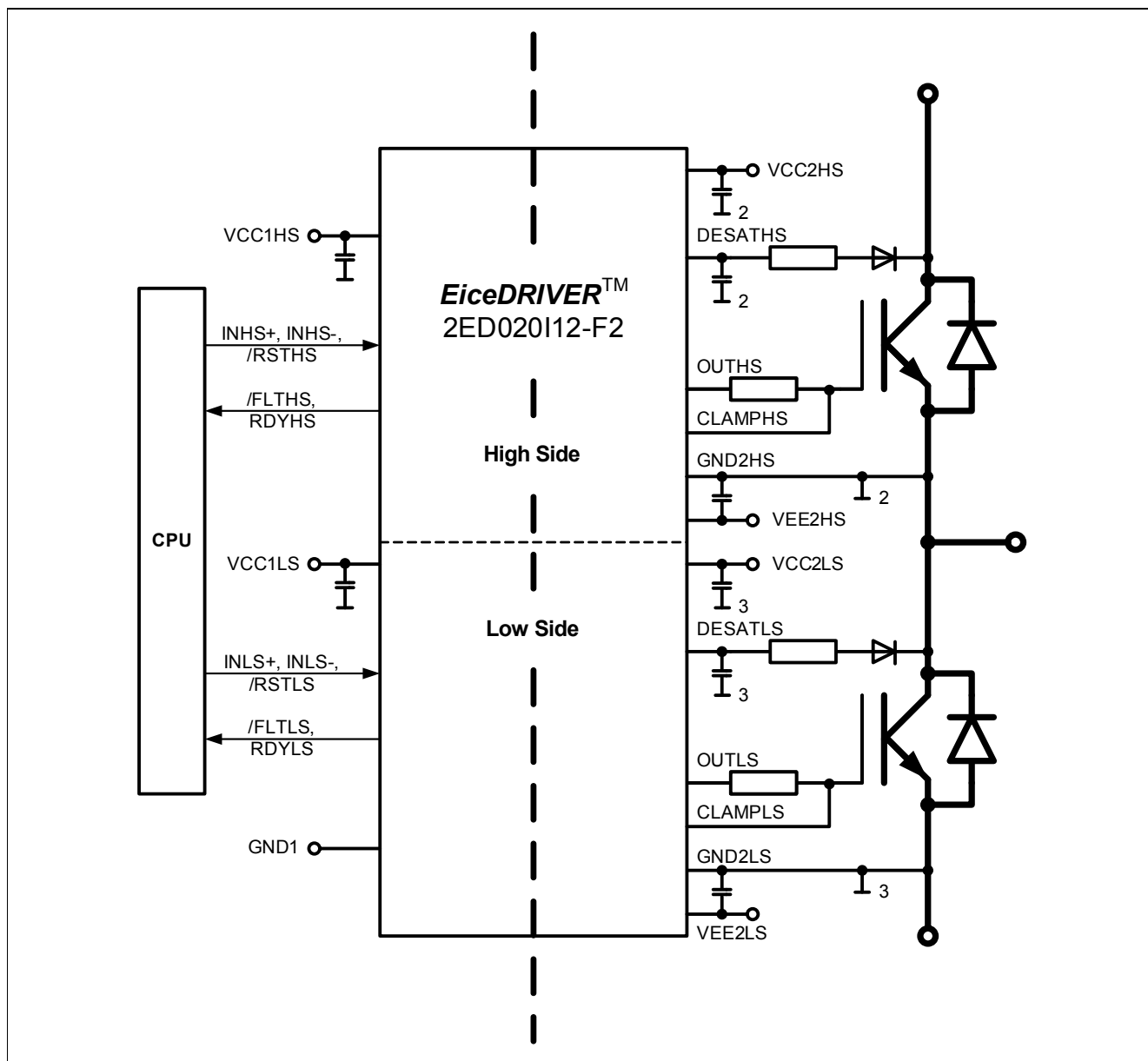
Figure 1 Typical Application
