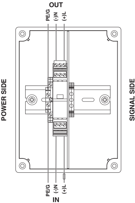
Connection diagram
