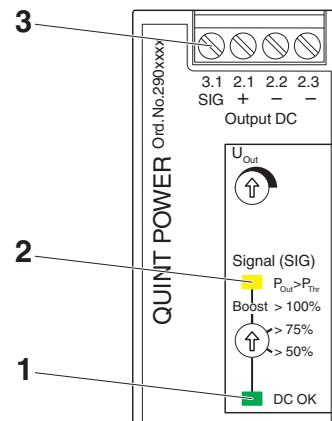
Figure 17 Position of signaling elements
