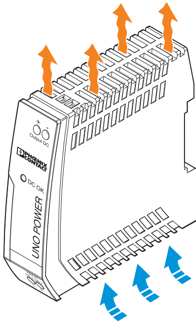
Figure 2 Convection
