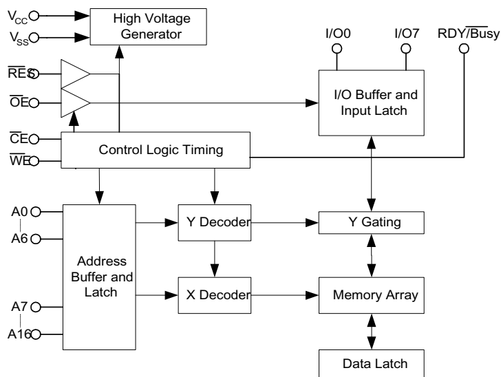
Logic Diagram
