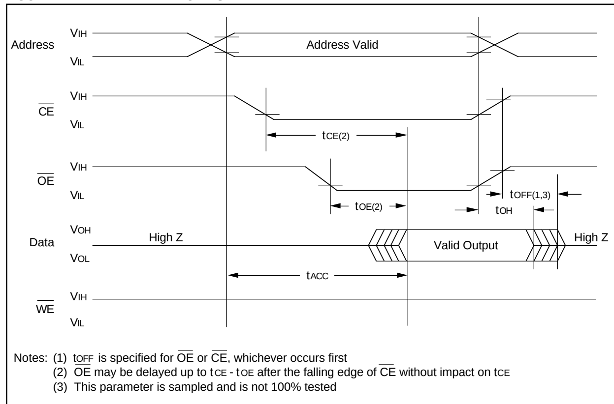
FIGURE 1-1: READ WAVEFORMS
