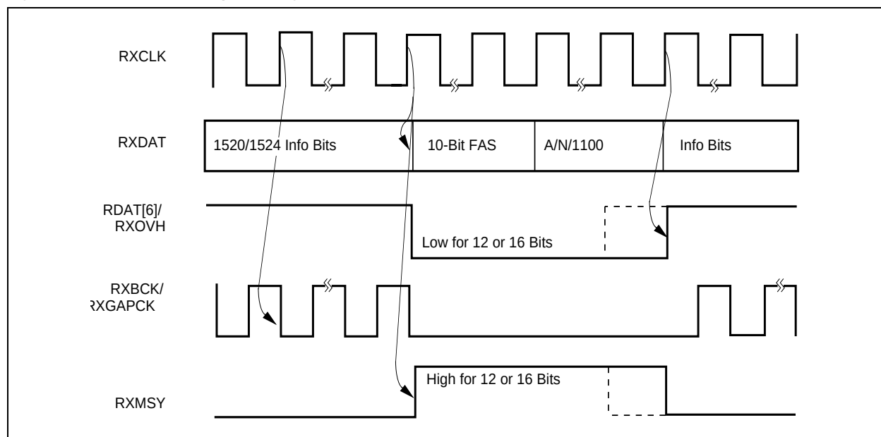
Figure 2-13. E3 Receiver Output Timing
