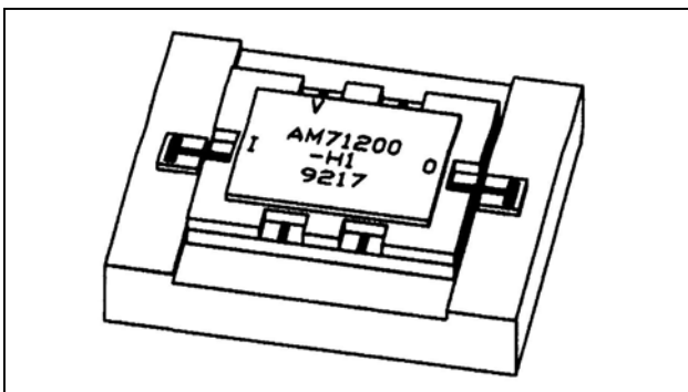
Figure 2. Fixtured MAAM71200-H1
