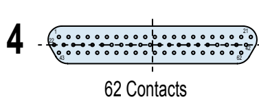
SOLDER CUP ORIENTATION
