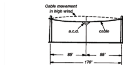
Fig. 1 – Level ground – 125'-170' spans
