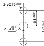
Panel Mounting Dimensions
