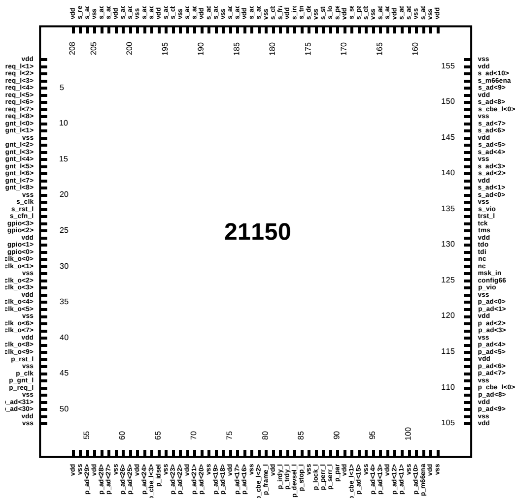
Figure 5. 21150 Pin Assignment
