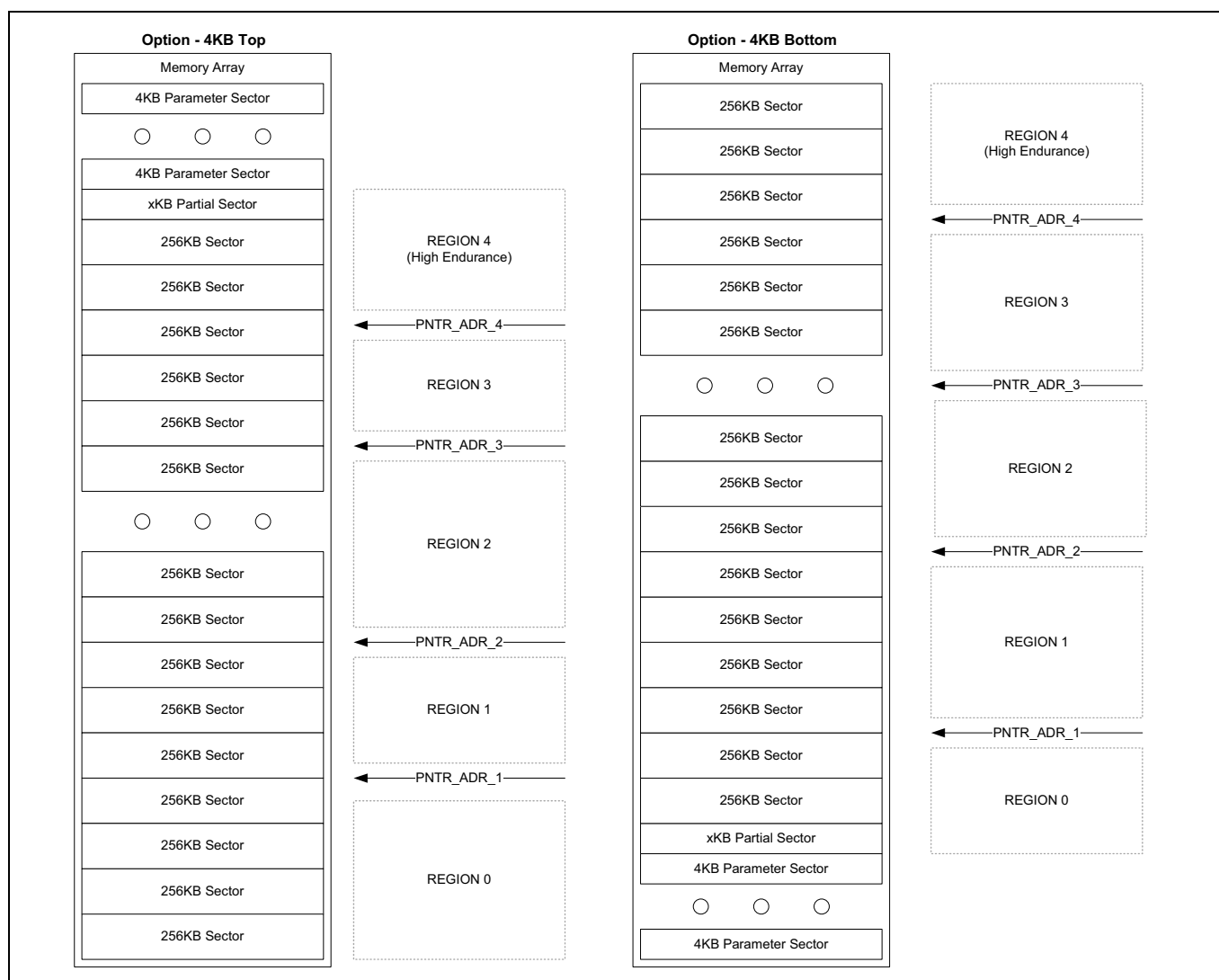
Figure 20 Infineon® Endurance Flex architecture overview
