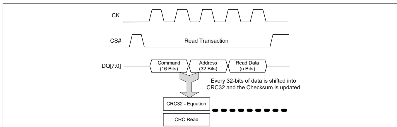
Figure 23 Read CRC protection
