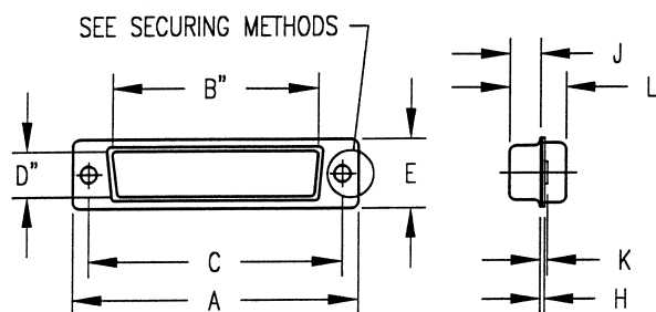
Plug Shell
