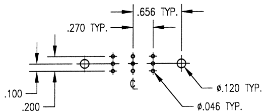
3W3 Straight Coax Contacts
