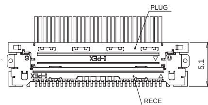
MATED VIEW
