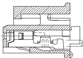
TERMINAL ASSEMBLY DRAWING
