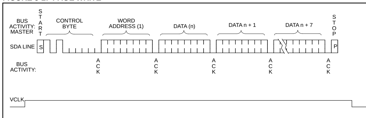
FIGURE 5-2: PAGE WRITE
