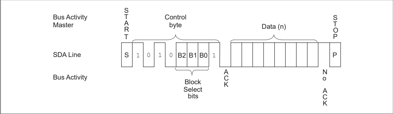
FIGURE 8-2: RANDOM READ
