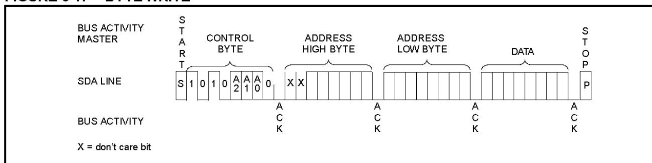
FIGURE 6-1: BYTE WRITE
