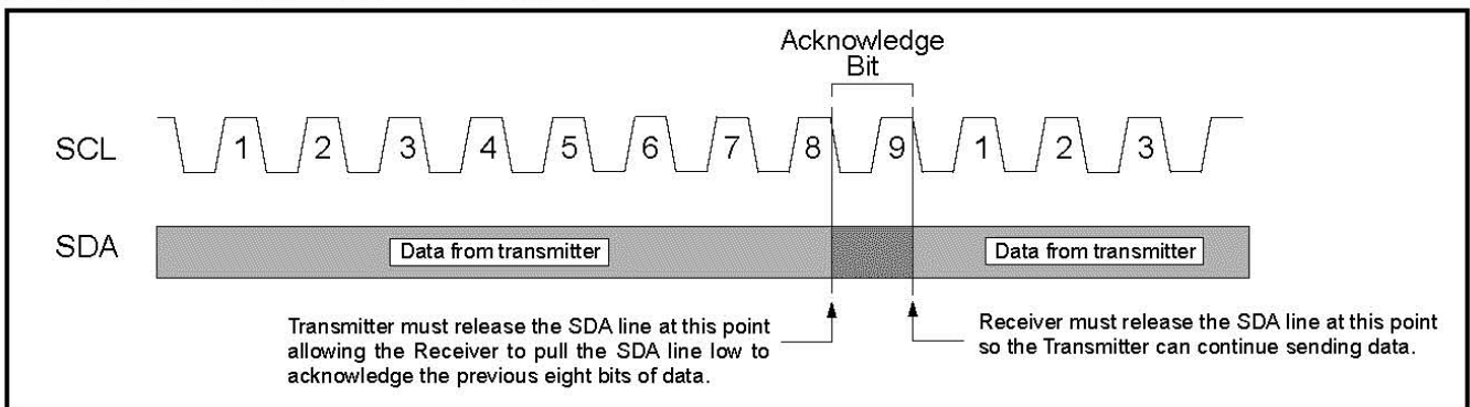
FIGURE 4-2: ACKNOWLEDGE TIMING
