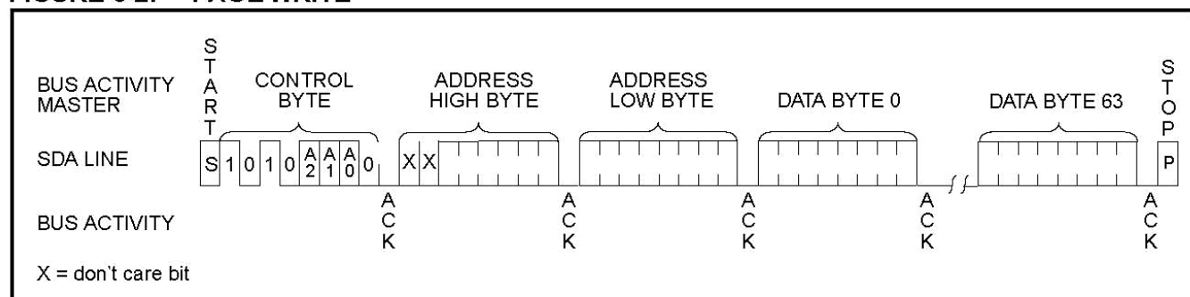
FIGURE 6-2: PAGEWRITE
