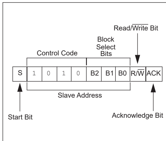
FIGURE 5-1: CONTROL BYTE ALLOCATION
