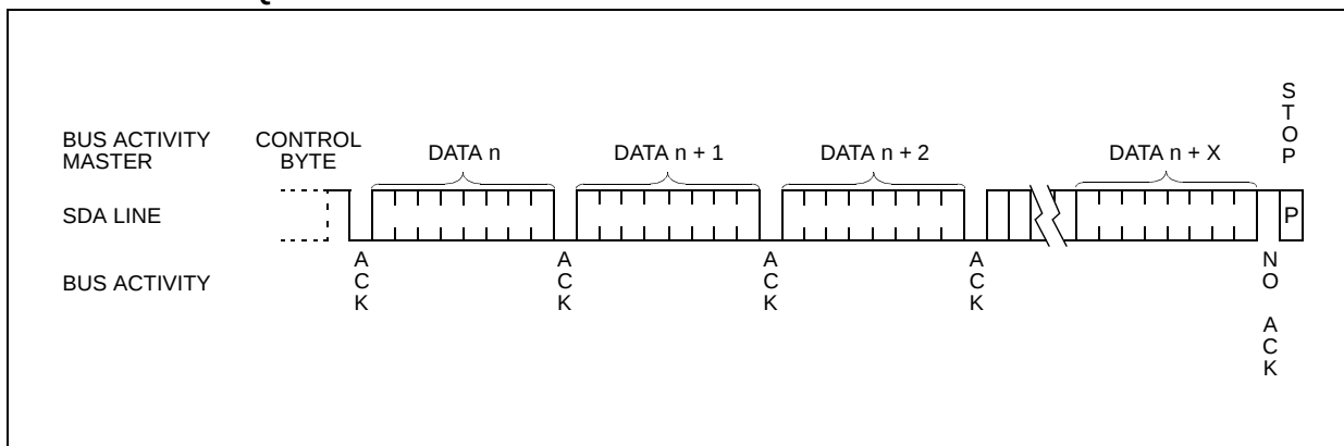
FIGURE 6-3: SEQUENTIAL READ
