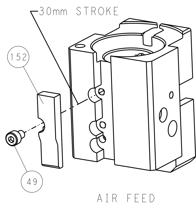
AIR FEED
