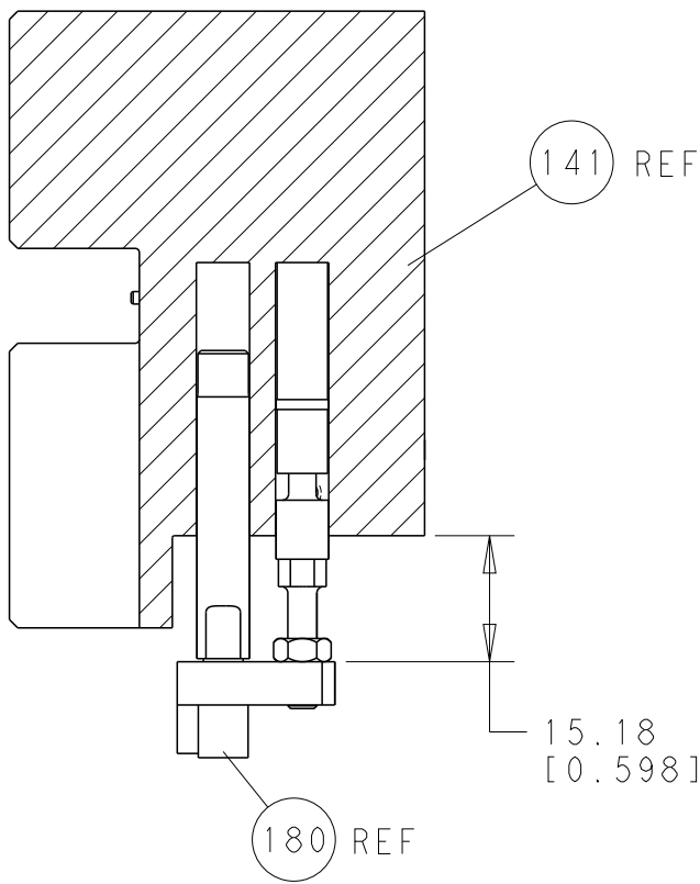
HOLDDOWN SET-UP
