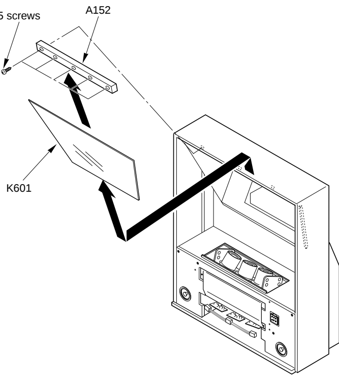
6 Mirror Removal
