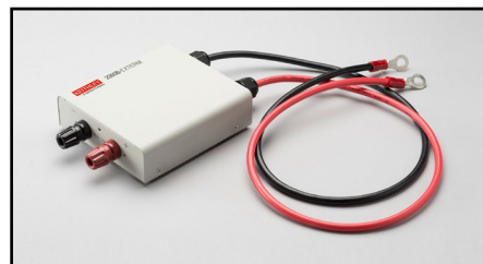
Model 2260B-EXTERM: Extended terminal; Test Leads, 0.7m (28 in.), and terminal box to bring outputs to the front of the instrument or another location. Magnetic base attaches to side of instrument.
