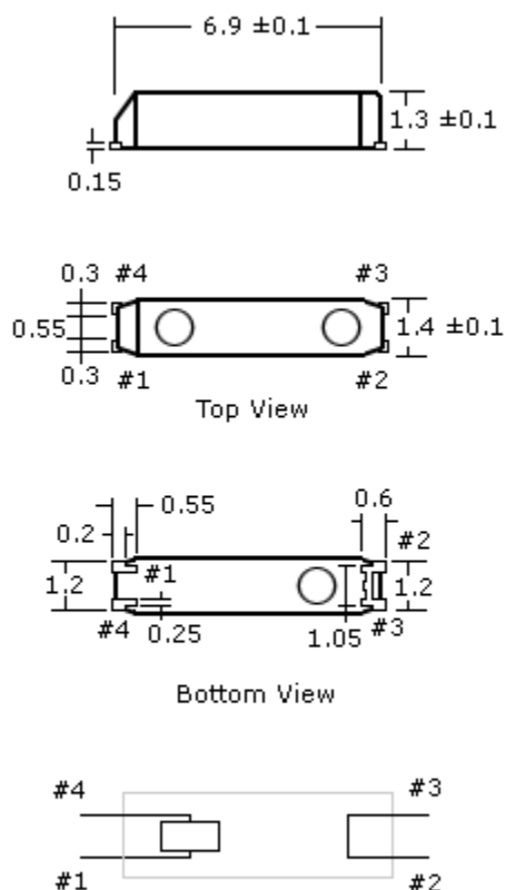
Figure 1) Pin Connection
