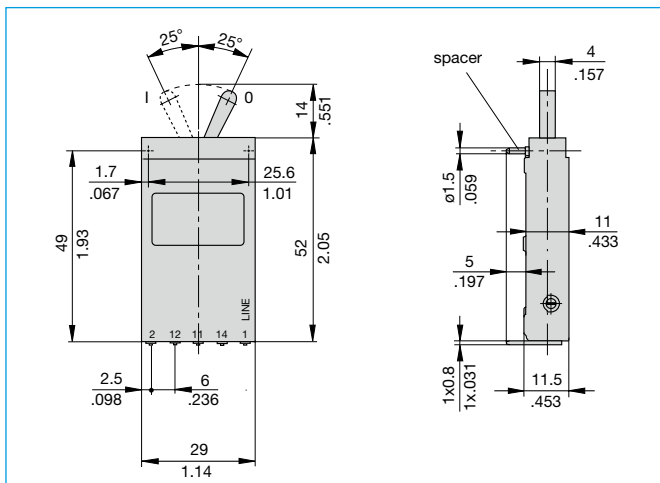
Dimensions 2215-G1..
