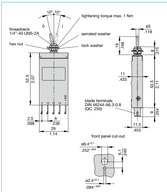
Dimensions 2215-G1..
