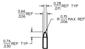
DETAIL Y SCALE 5:1 SEE NOTE 10
