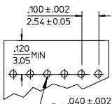
RECOMMENDED PC BOARD LAYOUT
