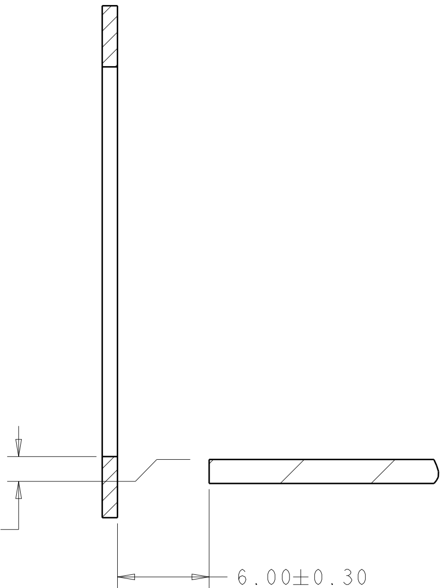
SECTION U-U
