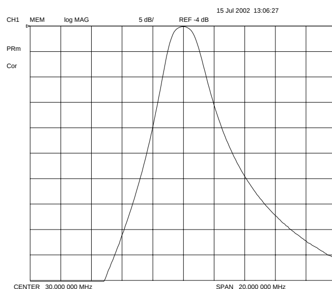
Overall Response (5 dB/div)
