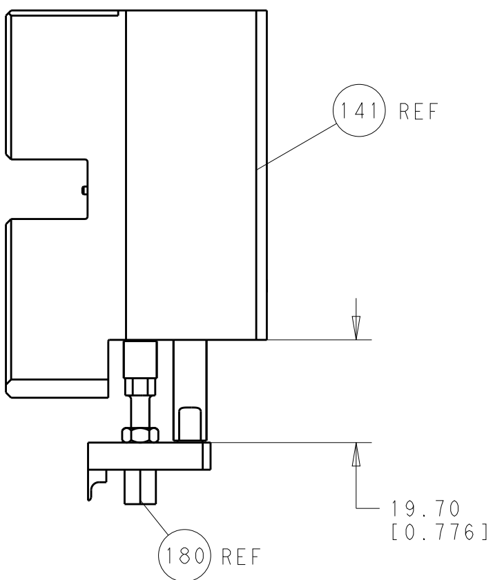
HOLDDOWN SET-UP
