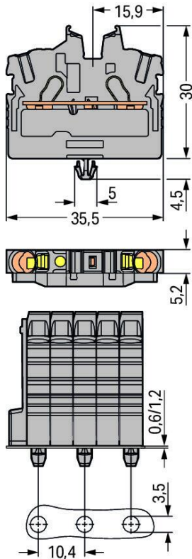
Modular terminal blocks and terminal strips with snap-in mounting feet
