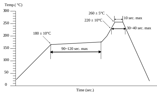
Reflow profile
