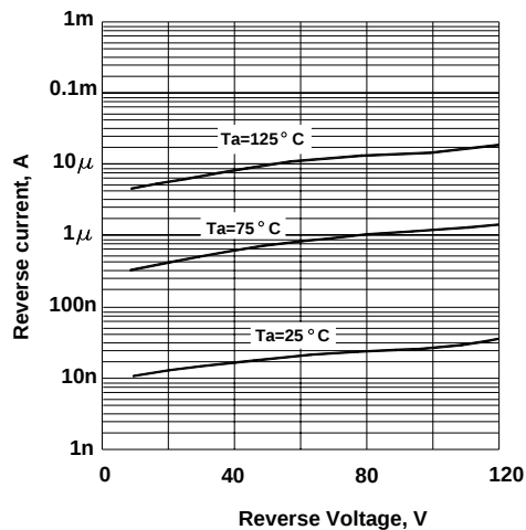
Reverse Characteristics
