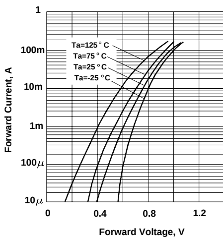
Forward Characteristics
