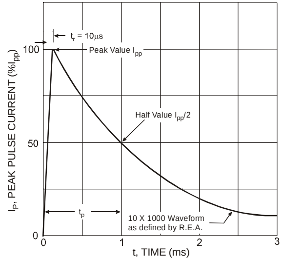
Figure 8 Pulse Waveform
