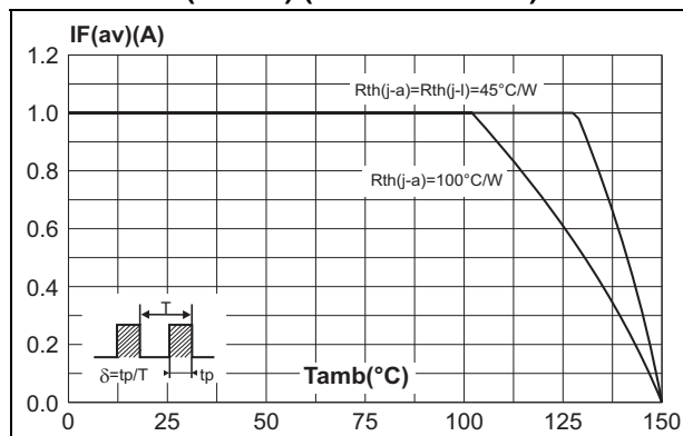
Figure 3. Average forward current versus ambient temperature (δ = 0.5) (1N5817/1N5818)
