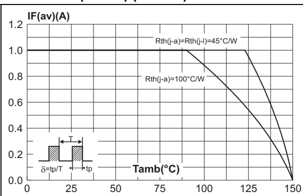
Figure 4. Average forward current versus ambient temperature (δ = 0.5) (1N5819)
