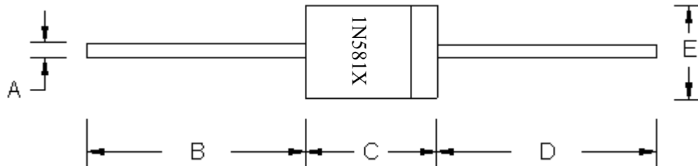
DO-41 Molded Plastic Package CYStek Package Code : LB
