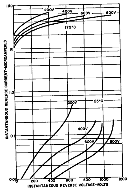
REVERSE CHARACTERISTICS
