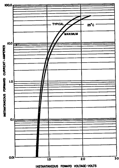
FORWARD CHARACTERISTICS
