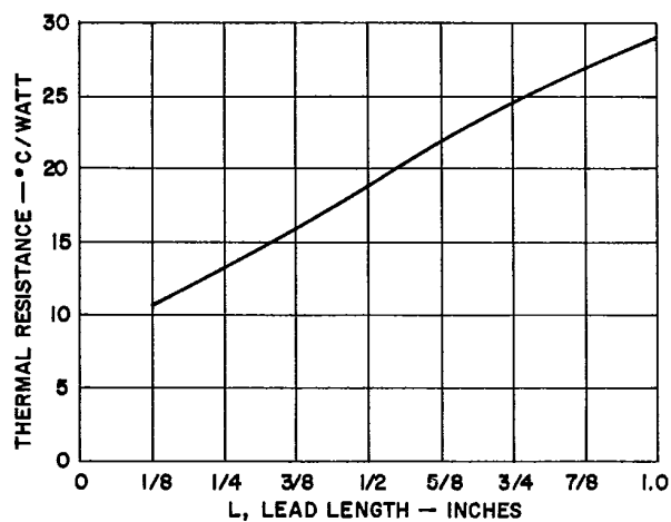
STEADY STATE THERMAL RESISTANCE
